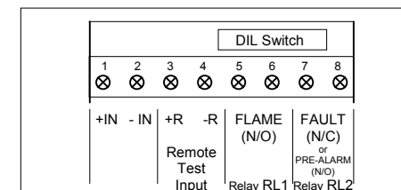
Fig. 1 Connection Terminals (Front Cover Removed)
